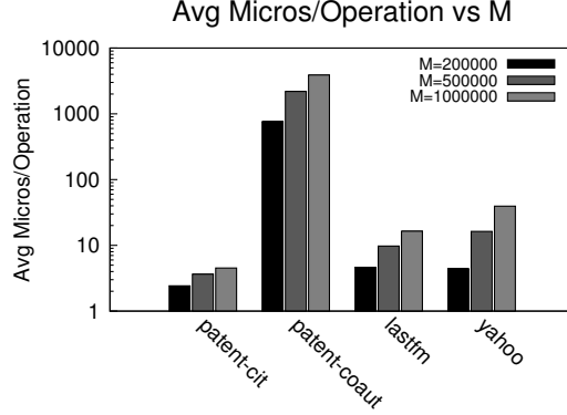
Figure 7: Trade-offs between the avg. update time ( \mu s ) and M for TRIÈST-FD.
