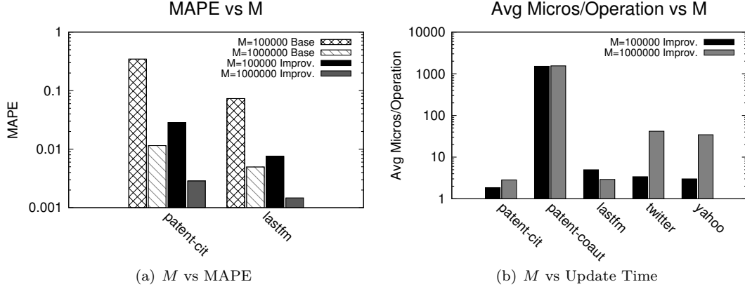
Figure 4: Trade-offs between M and MAPE or avg. update time ( \mu s ) – edge insertion only. Higher M implies lower errors but higher update times.
